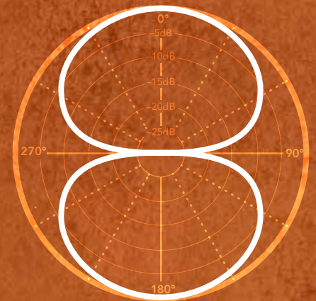
BI-DIRECTIONAL (FIGURE-8)
