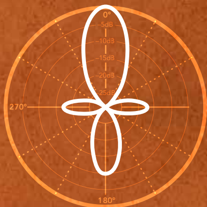
UNIDIRECTIONAL
